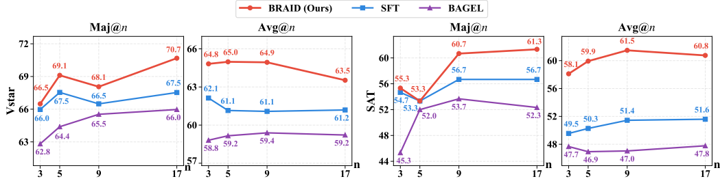
Figure 3: Maj@n and Avg@n curves on VStar and SAT benchmarks with varying number of samples n = \{3, 5, 9, 17\} . Complete results are available in Table 5.
