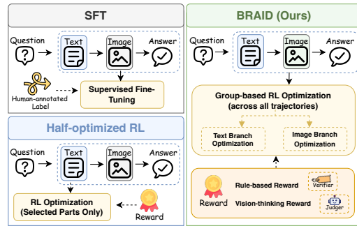
Figure 1: SFT, Half-optimized RL, and BRAID.
