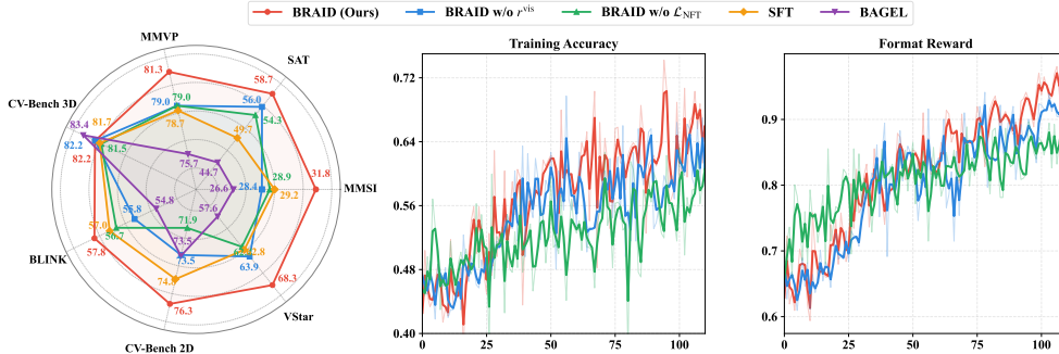
Figure 4: Ablation results. Left: Final test accuracy across seven benchmarks. Middle: Training average accuracy. Right: Training average format reward. Complete results are available in Table 4.
